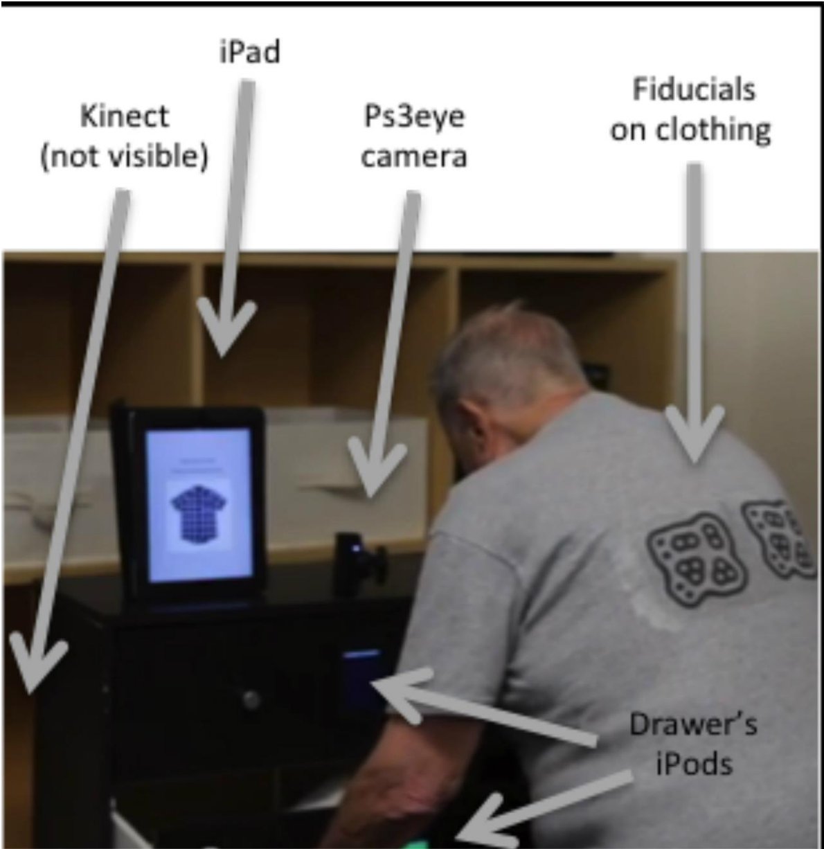
Figure 1. Typical human interaction with the DRESS system via an instrumented standard five-drawer dresser.
